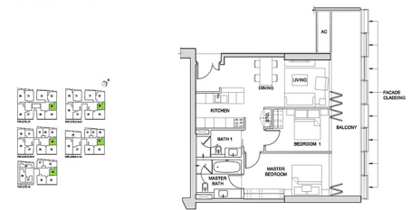
TYPE 2A1 (113 sq m / 1,216 sq ft)
